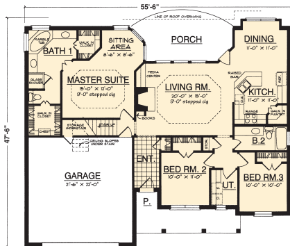
Main Floor
